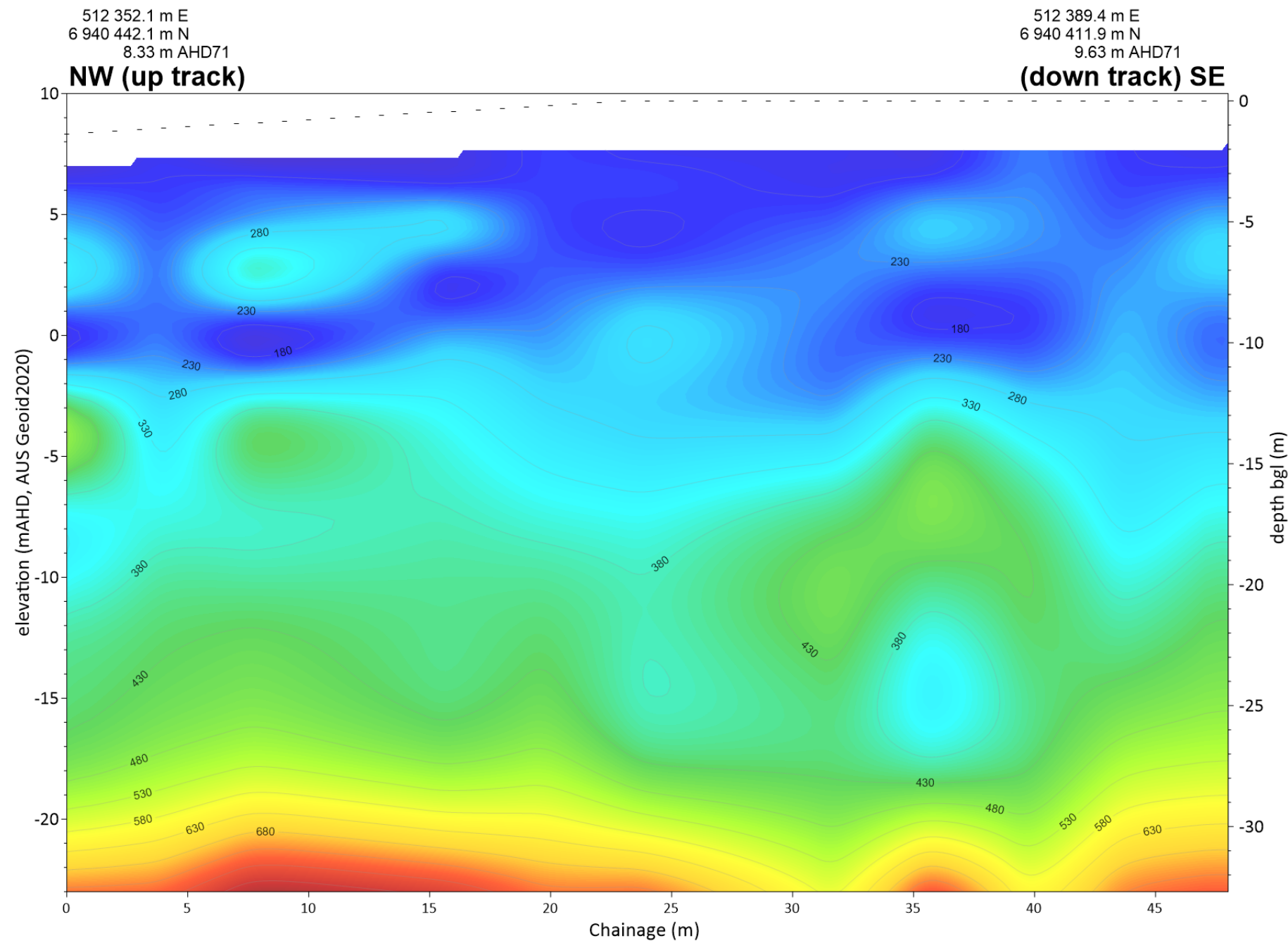
Seismic Line MASW AU-GP 143-2
